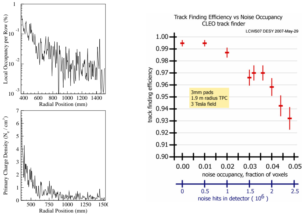
FIGURE 1.2. Occupancy for xyz = 1 \times 5 \times 5\text{mm}^3 voxels (left top) and space charge (left bottom) due to the major beam-beam effects (beamstrahlung photons, electron-positron pairs and neutrons) as simulated in [9]. Study of the tracking efficiency in the presence of backgrounds (right); this study [18] assumed a conservative voxel size of 3 \times 10 \times 40\text{mm}^3 .
