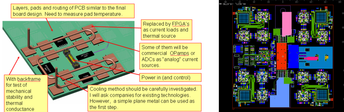
FIGURE 2.26. Left: Illustration of one section of the pad-board design. Right: One section of a test PCB with FPGAs, which mimic the pad PCB with the S-ALTR0 readout electronics, for the test of power delivery, power pulsing, and cooling. For pads of the size of 1.1 \times 4.5 \text{ mm}^2 , there are 12 identical sections on the test PCB.
