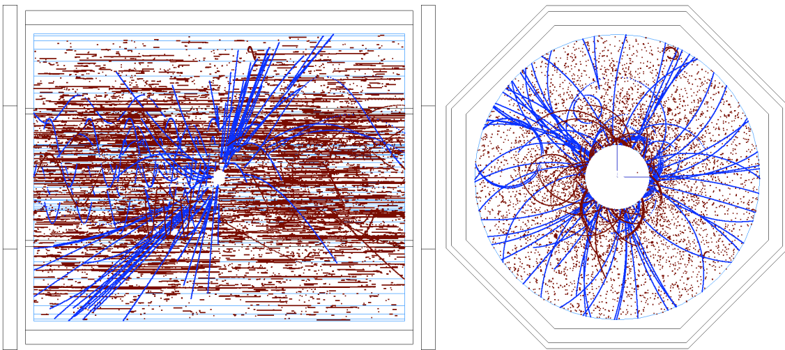
FIGURE 1.3. The rz and r\phi views of the TPC hits from a 500 GeV t\bar{t} event (blue) with 150 BXs of beam background (red) overlaid.
