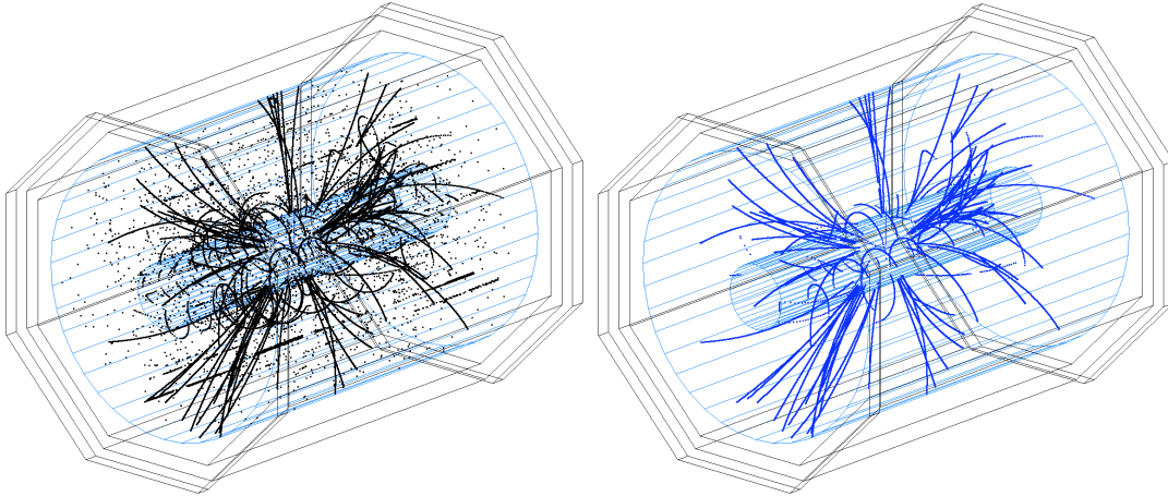
FIGURE 1.4. Left: The angle view with the micro-curler removal algorithm applied; this is the input to the TPC track finding algorithm. Right: the same event, now showing the reconstructed TPC tracks.
